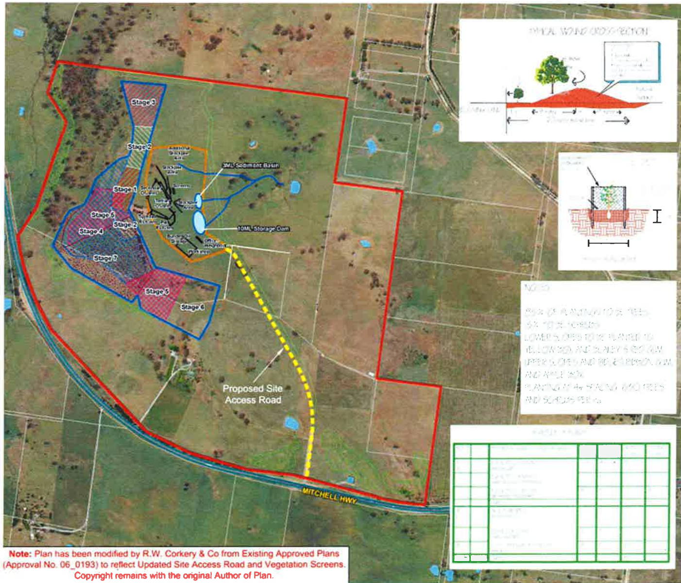
FIGURE 6 EAST GUYONG QUARRY PREFERRED PROJECT REHABILITATION PLAN
