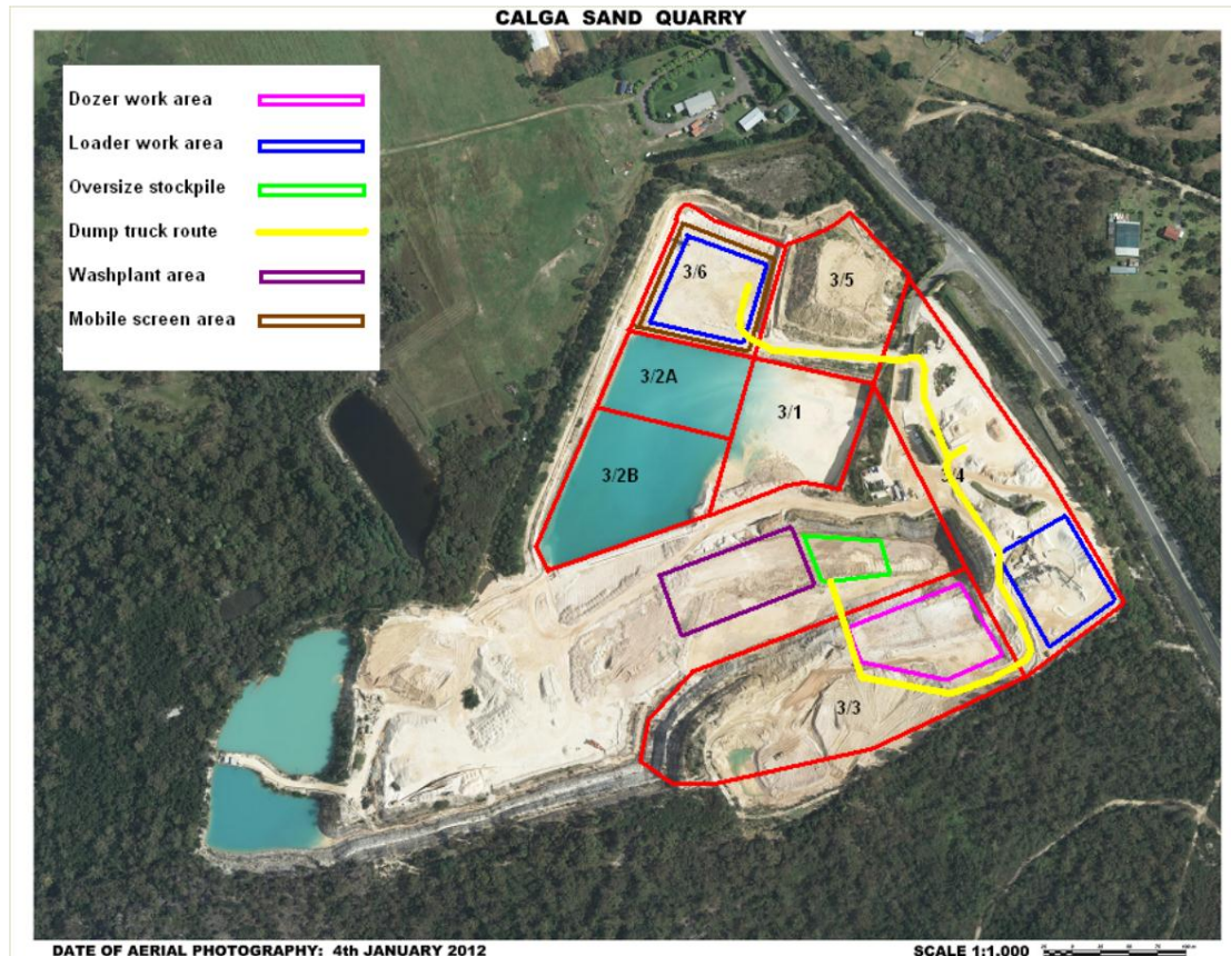
Figure 5-1 Quarry Site Layout and Operational Areas
